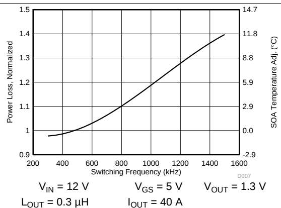
Figure 6. Normalized Power Loss vs Switching Frequency
