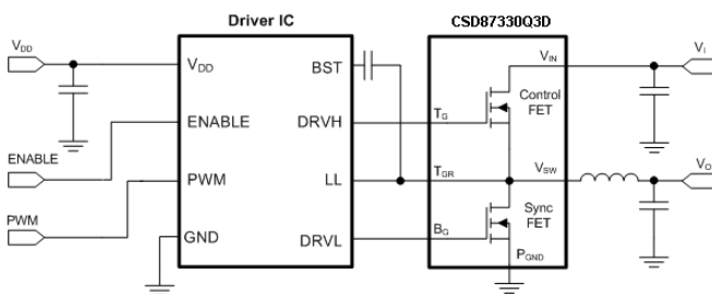
TYPICAL CIRCUIT
