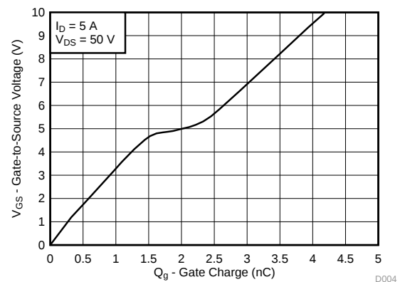
Gate Charge
