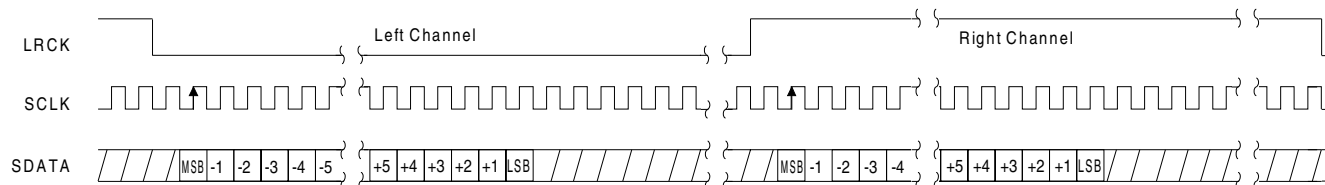
I 2 S, up to 24-Bit Data. Data Valid on Rising Edge of SCLK
