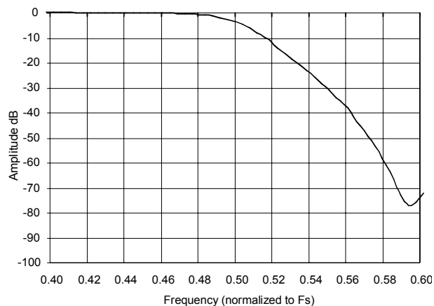
Figure 19. Interpolation Filter Double Speed Transition Band
