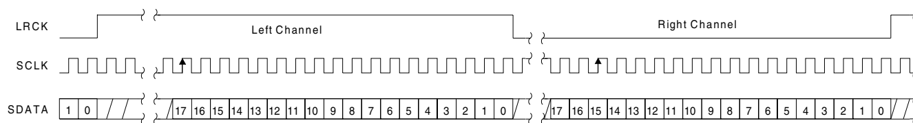
Right Justified, 18-Bit Data. Data Valid on Rising Edge of SCLK. SCLK Must Have at Least 36 Cycles per LRCK Period.
