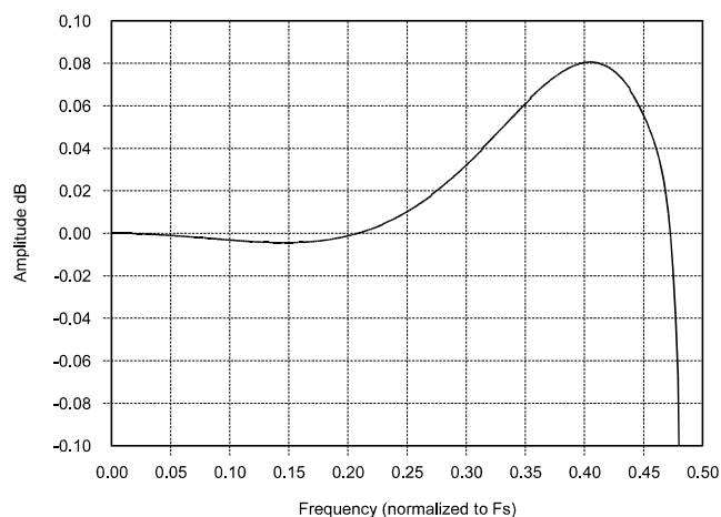
Figure 17. Interpolation Filter Single Speed Passband Ripple
