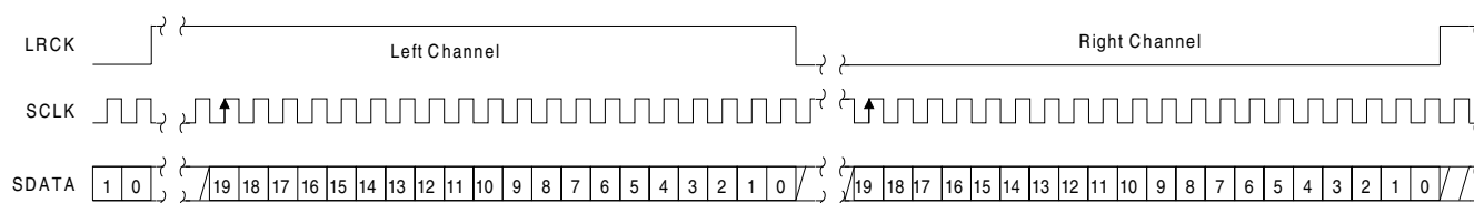
Right Justified, 20-Bit Data. Data Valid on Rising Edge of SCLK. SCLK Must Have at Least 40 Cycles per LRCK Period.
