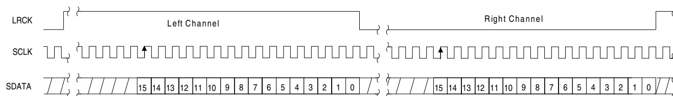
Figure 25. Left Justified, up to 24-bit data
