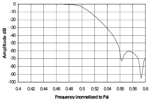
Figure 7. Decimation Filter Single Speed Transition Band
