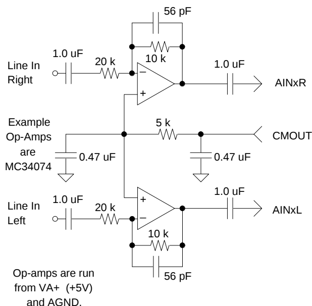
Figure 2 - Optional Line Input Buffer
