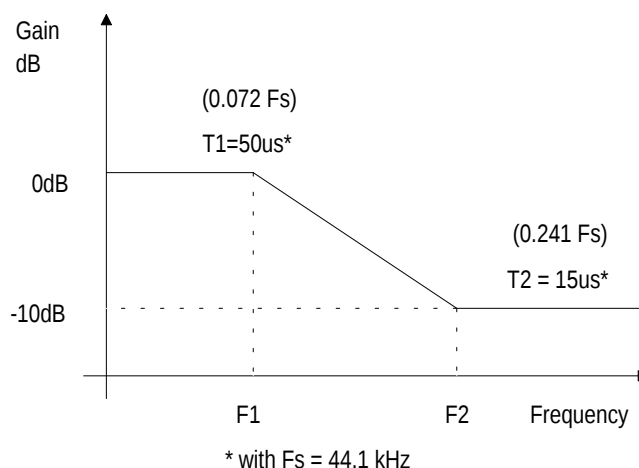
Figure 8 - De-emphasis Curve.
