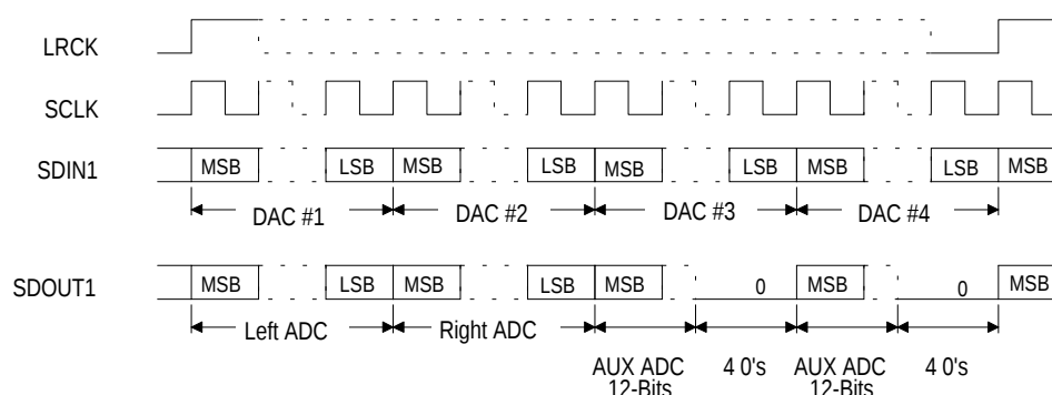
Figure 5 - One data line mode (Format 4)
