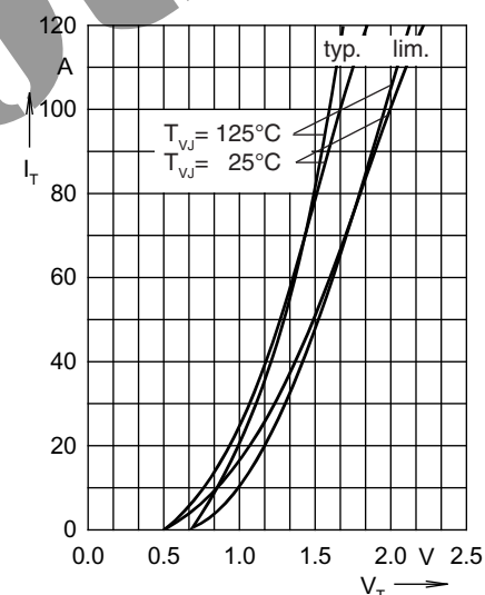
Fig. 3 On-state characteristics
