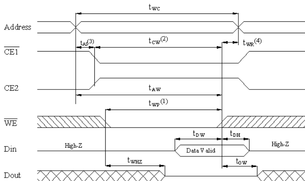
WRITE CYCLE 2. (CE1 and CE2 Controlled)
