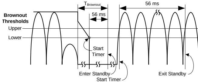
Figure 17. Brownout Sequence
