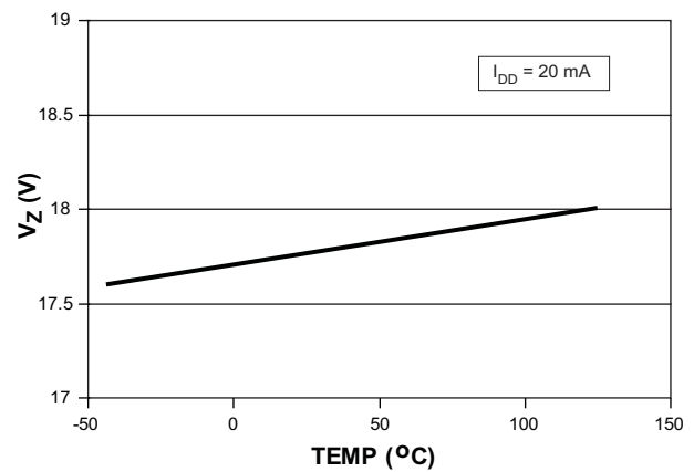
Figure 4. V_{DD} Zener Voltage vs. Temp
