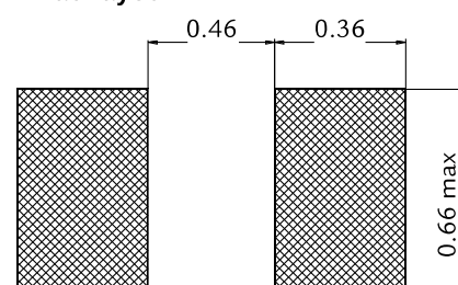
Pad layout
