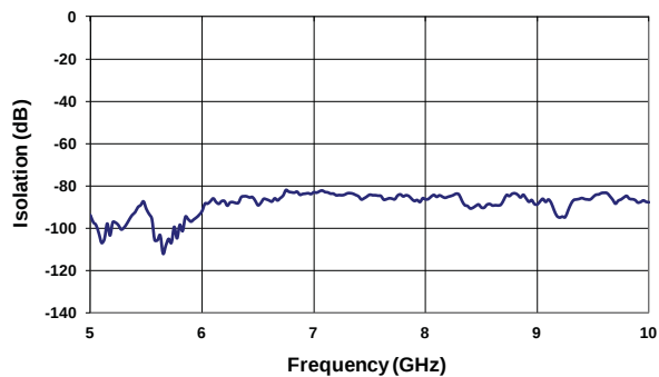
Isolation (5-10 GHz)
