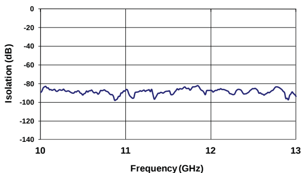
Isolation (10-13 GHz)
