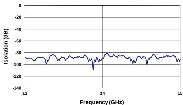
Isolation (13-15 GHz)
