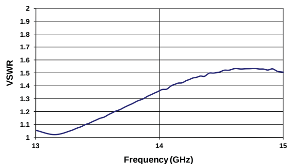
VSWR (13-15 GHz)
