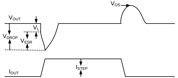
Figure 23. Typical Output Voltage Response Waveform.
