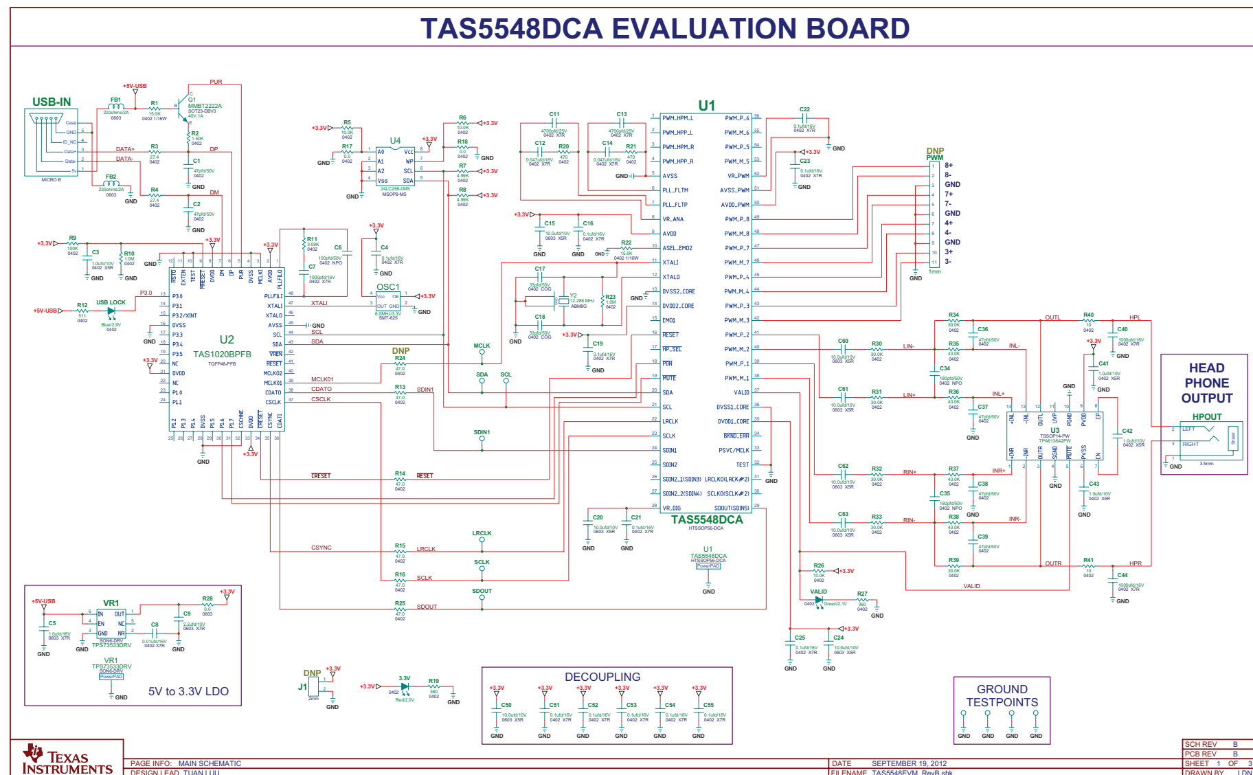
Figure 11. TAS5548EVM Schematic
