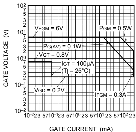
GATE CHARACTERISTICS
