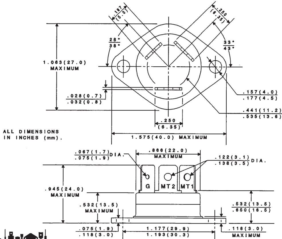
MECHANICAL OUTLINE
