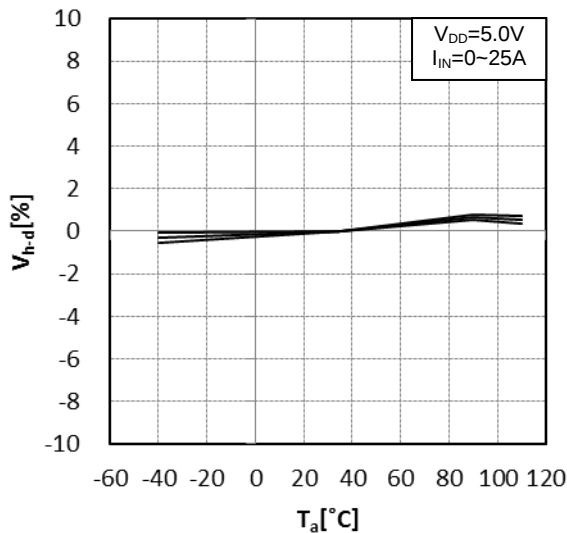
Figure 6. Temperature drift of sensitivity (for reference, n=3)
