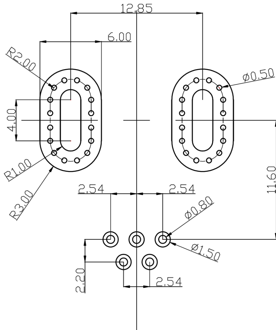
Figure 10. Recommended land pattern of CQ-236B
