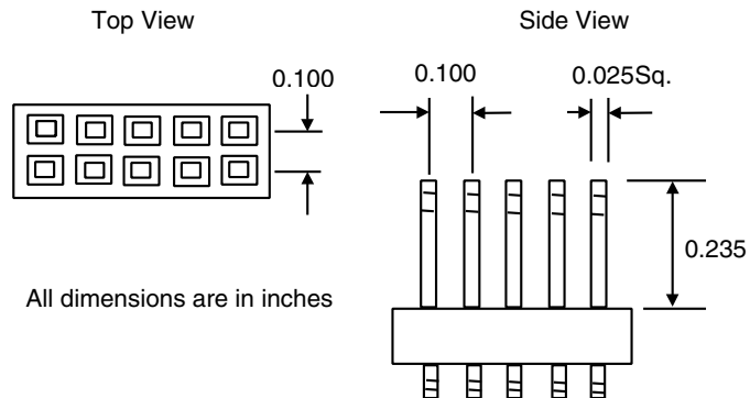
Figure 2-4. 10-pin Male Header Dimensions
