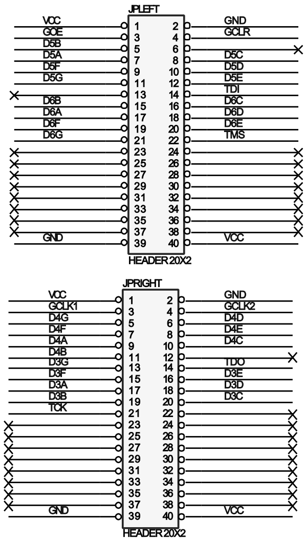
Figure 4-2. Schematic Diagram of 44-pin PLCC Socket Adapter Board
