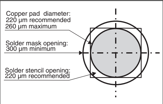
Figure 8. Footprint
