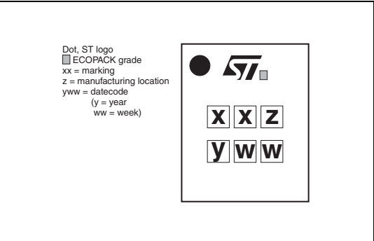
Figure 9. Marking
