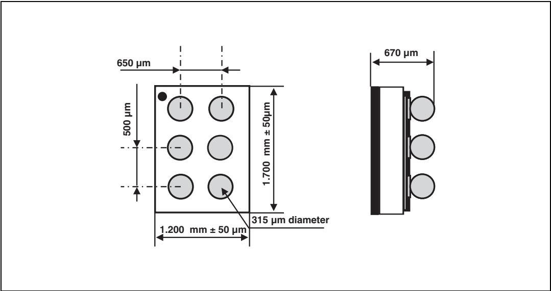
Figure 6. Package dimensions
