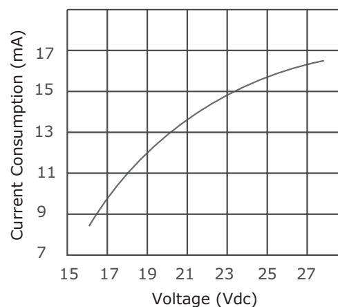
Voltage vs. Current Consumption at 25°C
