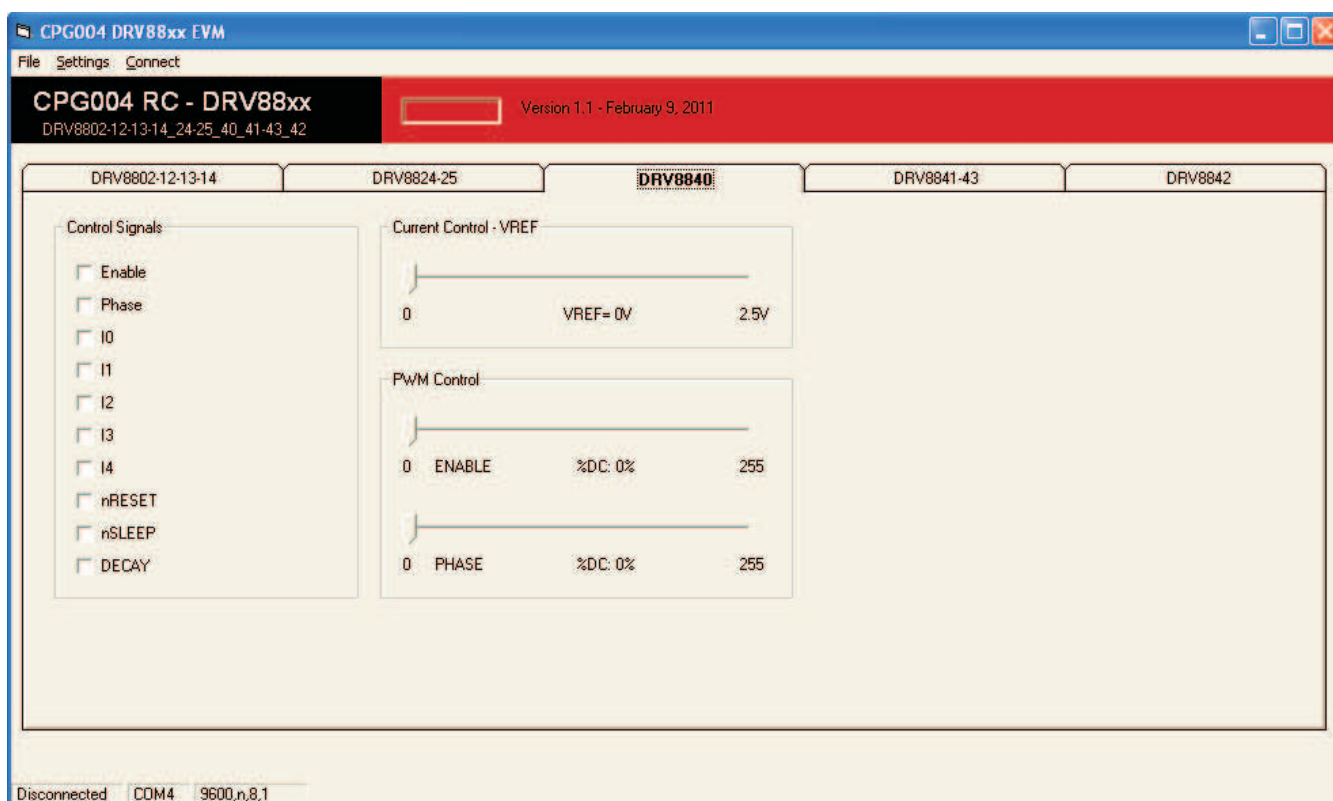
Figure 3. DRV8840 Tab
