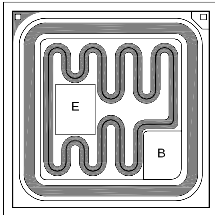
BACKSIDE COLLECTOR
