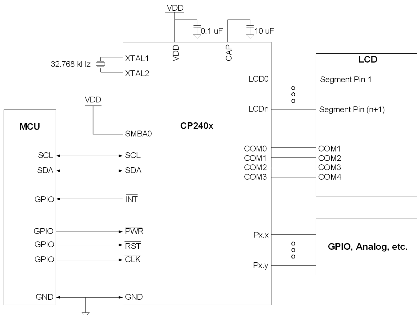
Figure 1.6. Typical Connection Diagram (SMBus/I²C Interface)
