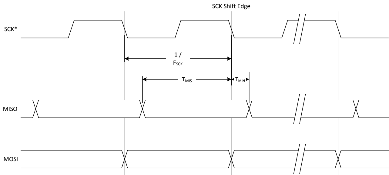
Figure 5. SPI Master Timing (CPHA=Leading Edge)
