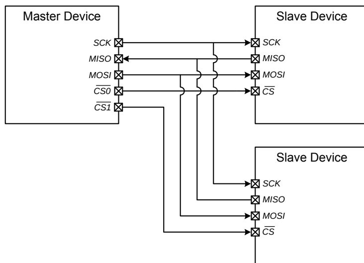
Figure 3. 4-Wire Single Master Mode and 4-Wire Slave Mode Connection Diagram
