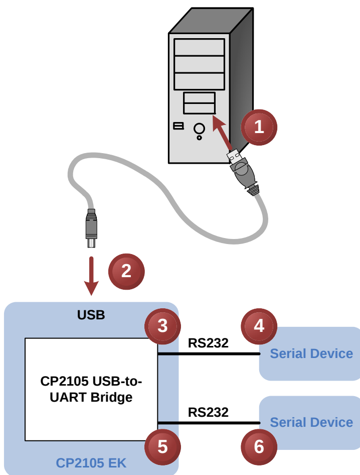
Figure 1. Hardware Setup
