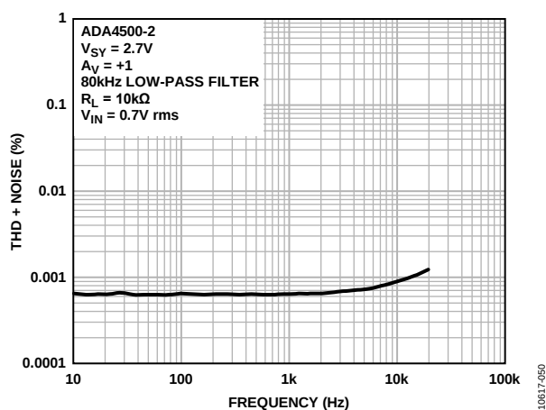
Figure 56. THD + Noise vs. Frequency, V_{SV} = 2.7\text{ V}
