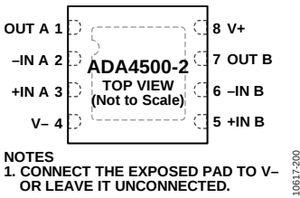
Figure 4. 8-Lead LFCSP Pin Configuration
