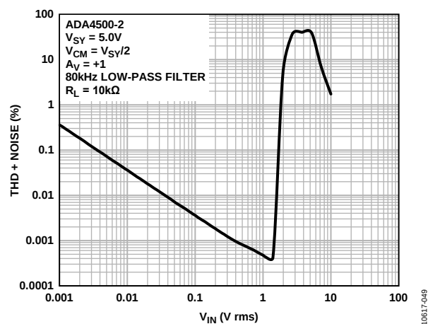
Figure 57. THD + Noise vs. Amplitude, V_{SV} = 5.0\text{ V}
