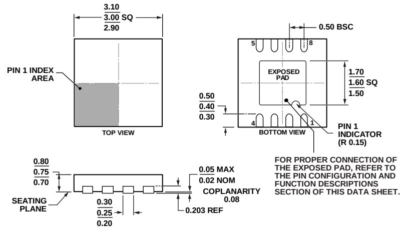
Figure 67. 8-Lead Lead Frame Chip Scale Package [LFCSP_WD] 3 mm × 3 mm Body, Very, Very Thin, Dual Lead (CP-8-12)
