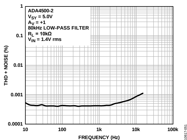
Figure 58. THD + Noise vs. Frequency, V_{SV} = 5.0\text{ V}
