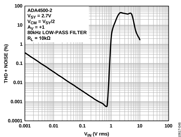
Figure 55. THD + Noise vs. Amplitude, V_{SV} = 2.7\text{ V}
