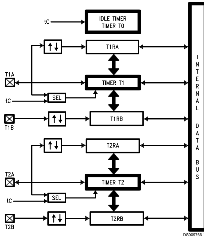
FIGURE 7. Timers
