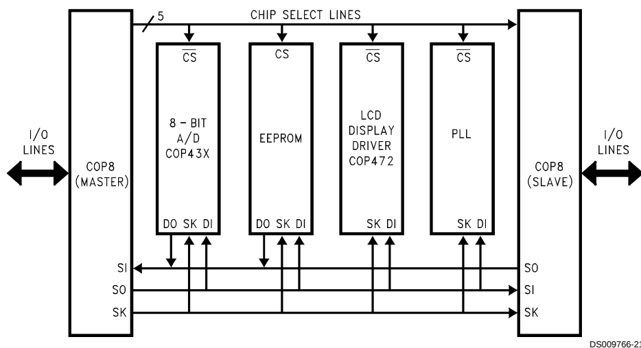
FIGURE 14. MICROWIRE/PLUS Application
