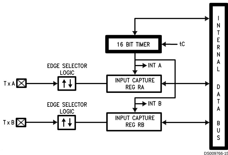
FIGURE 10. Timer in Input Capture Mode
