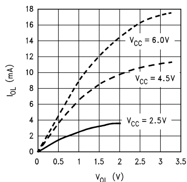
Port L/C/G Push-Pull Sink Current
