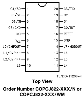
FIGURE 3. Connection Diagrams
