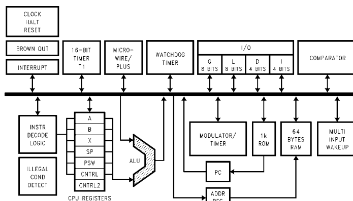
FIGURE 1. Block Diagram
