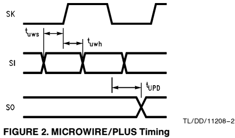
FIGURE 2. MICROWIRE/PLUS Timing
