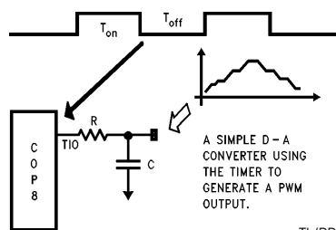
FIGURE 11. Timer Application
