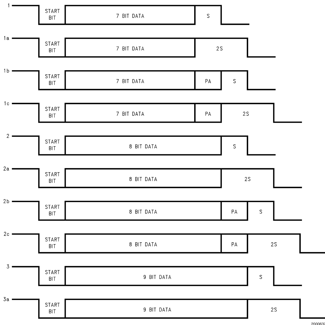
FIGURE 22. Framing Formats
