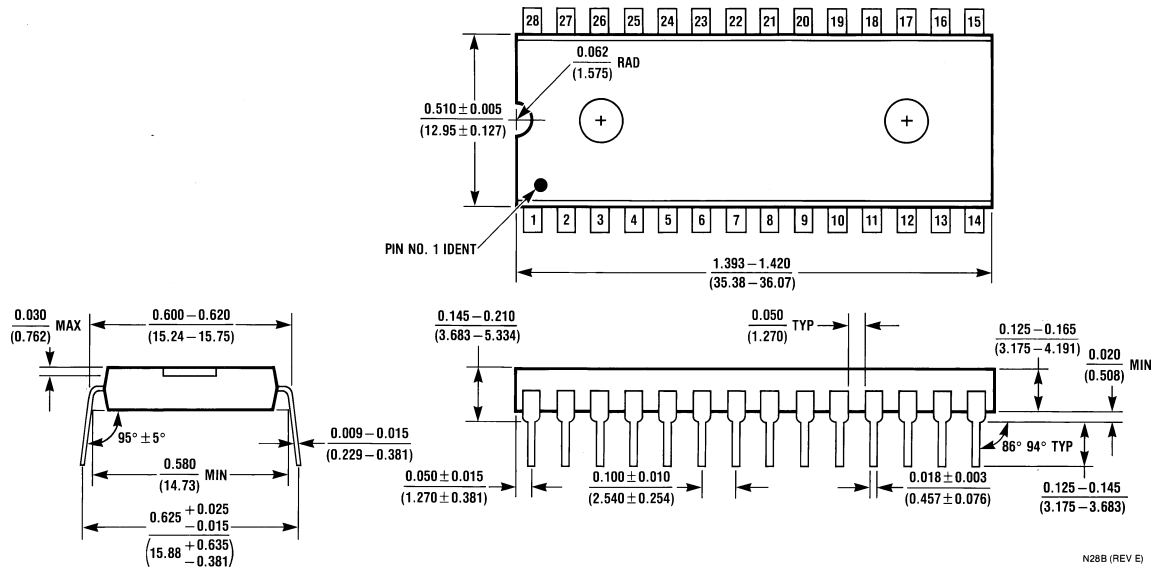
Molded Dual-In-Line Package (N) Order Number COP8AME9ENA8 NS Package Number N28B
