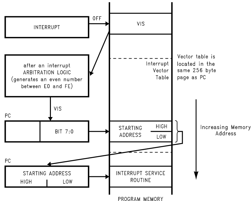
FIGURE 32. VIS Operation
