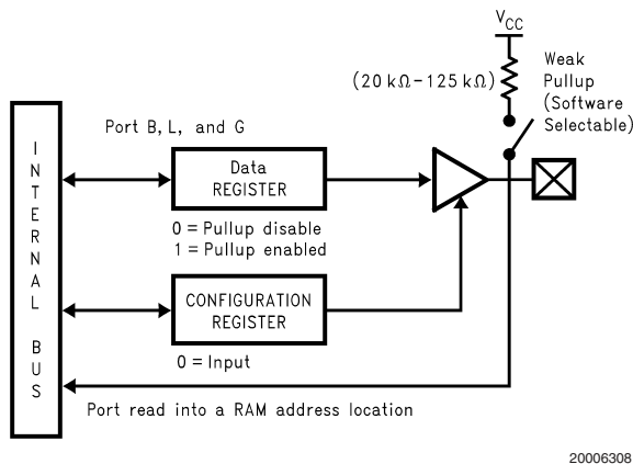
FIGURE 4. I/O Port Configurations—Input Mode
