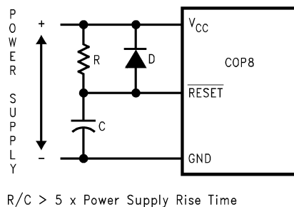
FIGURE 8. Reset Circuit Using External Reset
