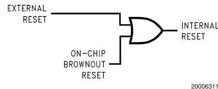
FIGURE 7. Reset Logic
