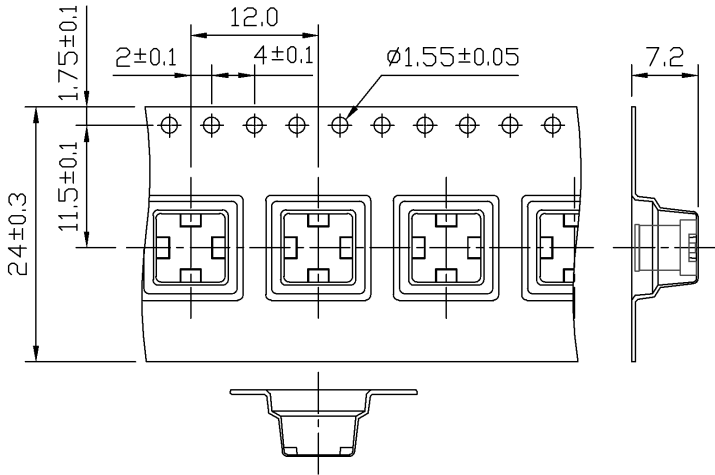
TAPE DIMENSIONS
