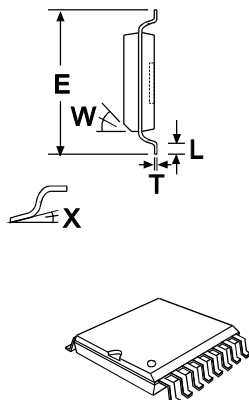
Figure 12 : 16-pin SOIC (D4) Mechanical Outline: Order as part no. CMX602AD4
