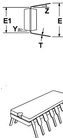
Figure 13 : 16-pin DIL (P3) Mechanical Outline: Order as part no. CMX602AP3
