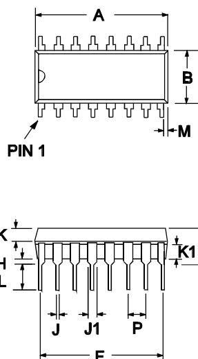
Figure 13 : 16-pin DIL (P3) Mechanical Outline: Order as part no. CMX602AP3
