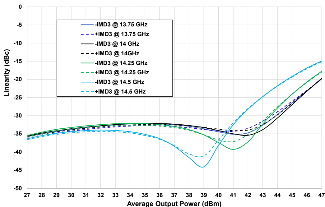
Figure 4. - CMPA1D1E080F Two Tone Power Sweep IMD3 @ 1 MHz Carrier Spacing vs Output Power V_{DD} = 40\text{ V} , I_{DQ} = 640\text{ mA} , Tcase = 25°C
