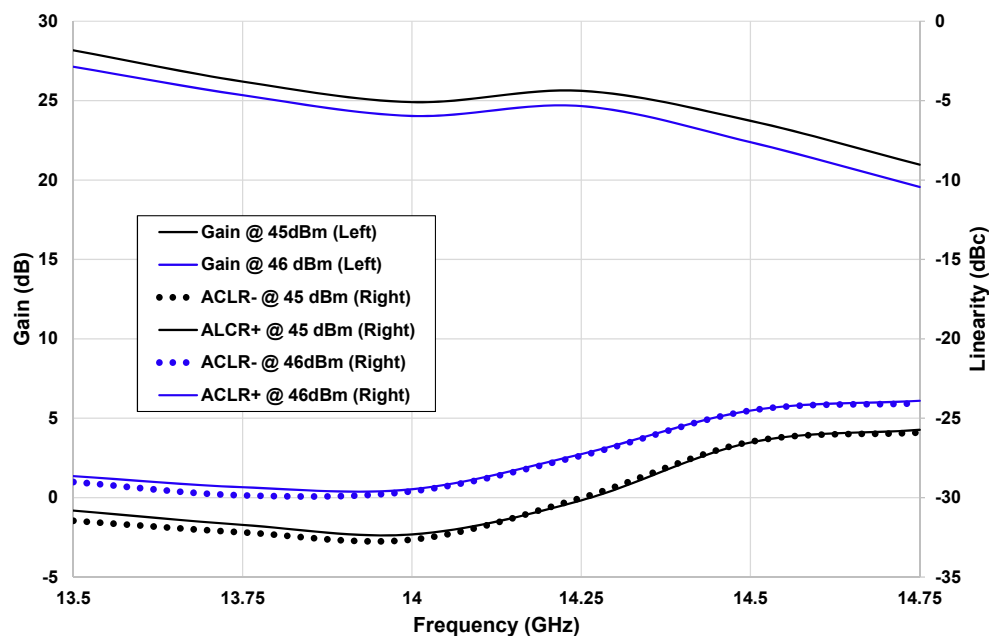
Figure 3. - ACLR and Gain vs Frequency at P_{AVE} = 45 and 46 dBm, OQPSK Modulation, 1.6 Msps, PN23, Alpha Filter = 0.2 V_{DD} = 40\text{ V} , I_{DQ} = 640\text{ mA} , Temp = 25°C
