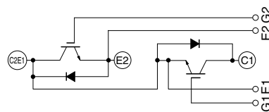
CIRCUIT DIAGRAM
