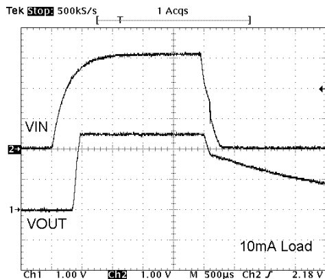
Cold Start Power-Up/Down with 10mA Load
