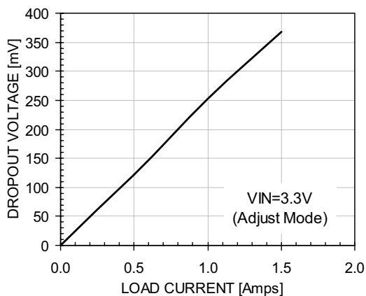
Dropout Voltage with Load
