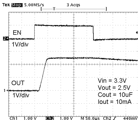
Enable Power-Up with 10mA Load
