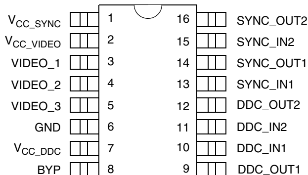
16 Pin QSOP
