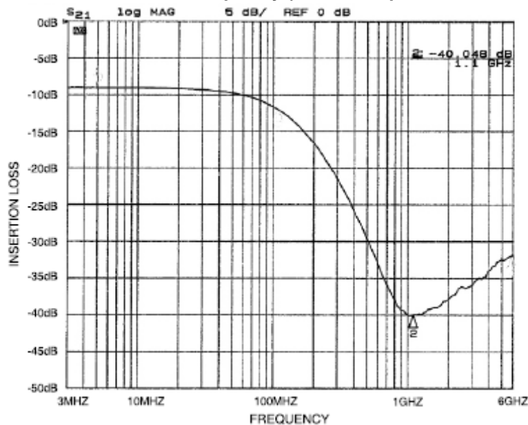
Figure 18. Insertion Loss vs. Frequency (FILTER8 Input to GND, CM1636-08DE)
