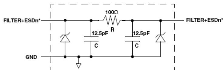
1 of 8 EMI/RFI + ESD Channels
