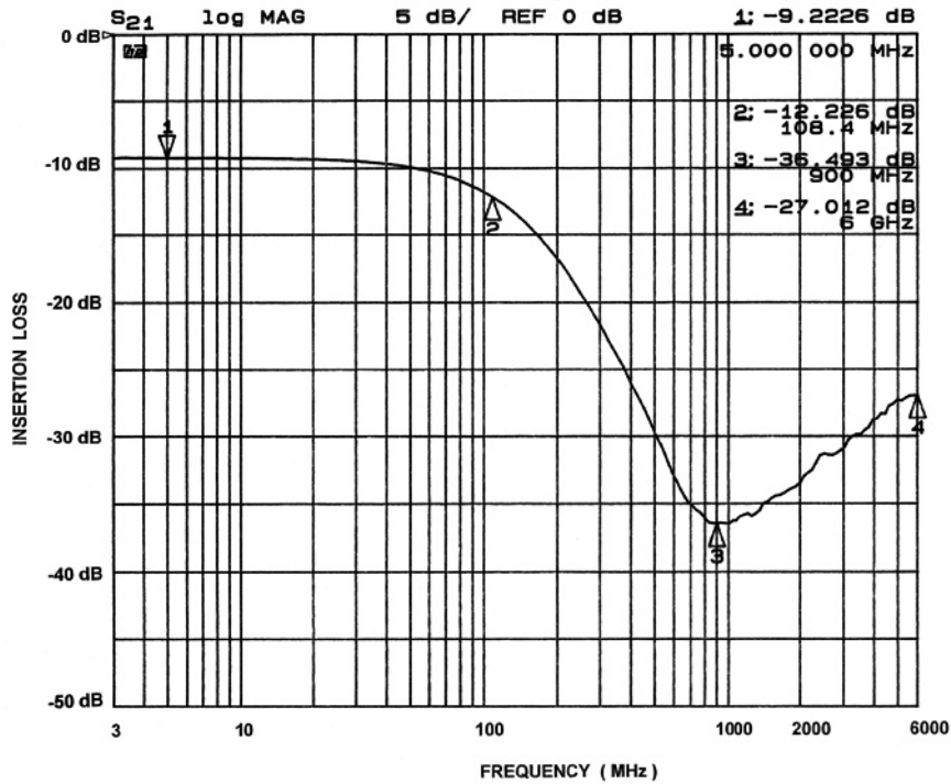
Figure 10. Channel 5 EMI Filter Performance (CM1436-06/08 Only)
