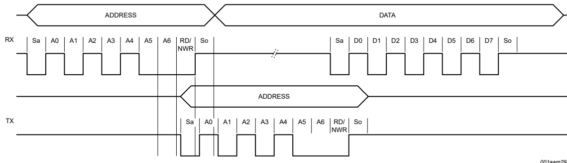
Figure 15. Example diagram for a UART write
