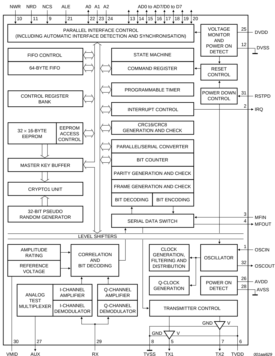
Fig 1. CLRC632 block diagram
