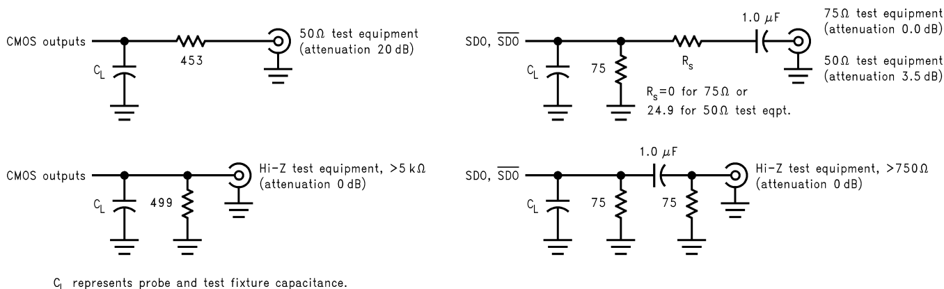
Figure 2. Test Loads
