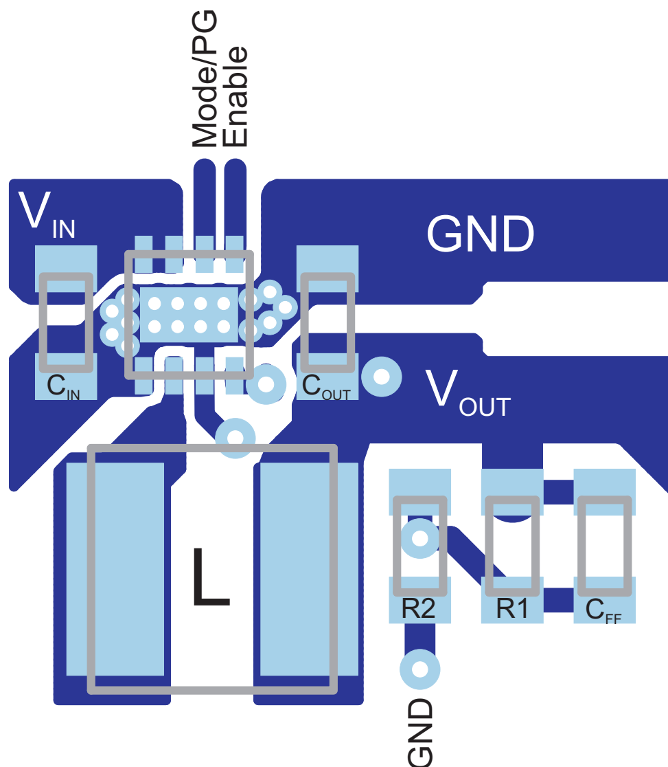
Figure 28. PCB Layout
