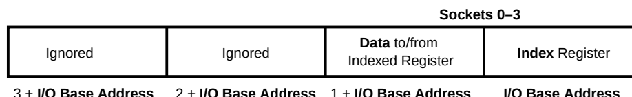
Figure 7-1. Operation Registers as PCI Doubleword I/O Space at I/O Base Address Register (Programmed at Configuration Space, Offset 44h)
