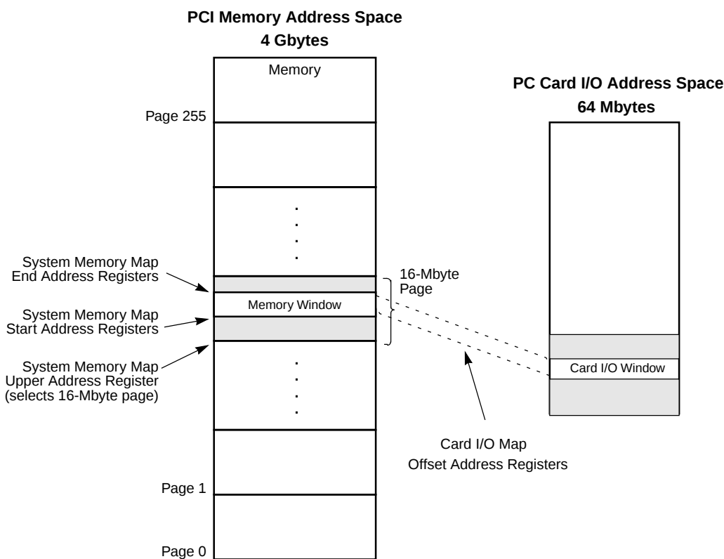
Figure 3-3. Memory-to-I/O Window Organization
