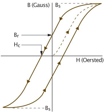
Figure 2. B-H Loop
