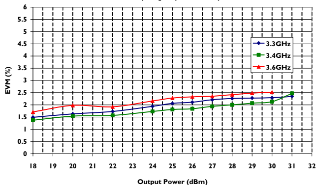
EVM Vs Output Power Vs Frequency OFDM 802.16d, 64QAM, PAR=9dB, +12V
