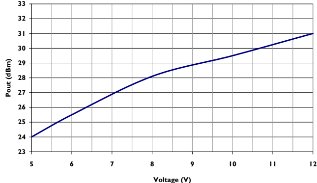
Pout @ EVM < 2.5% Vs Voltage 3.4GHz
