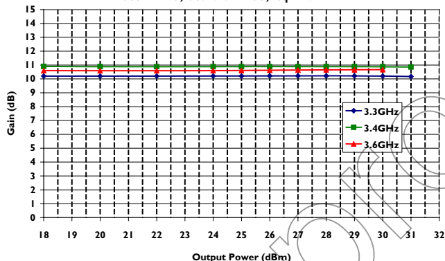
Gain Vs Output power Vcc = +12V, Vcontrol = +5V, Icq = 167mA
