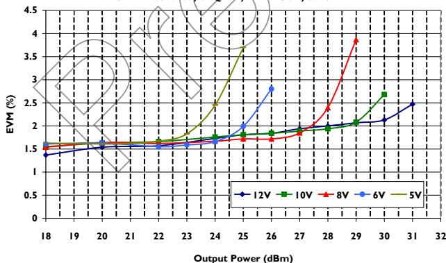
EVM Vs Output Power Vs Voltage OFDM 802.16d, 64QAM, PAR=9dB, 3.4GHz
