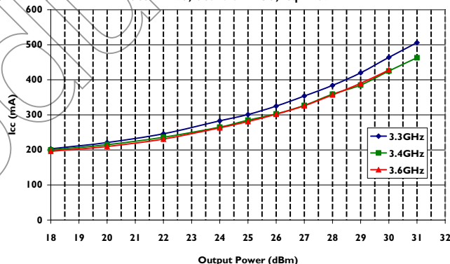
Current Vs Output power Vs Frequency Vcc = +12V, Vcontrol = +5V, Icq = 167mA
