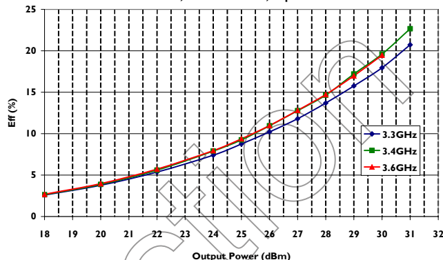
Efficiency Vs Output power Vs Frequency Vcc = +12V, Vcontrol = +5V, Icq = 167mA
