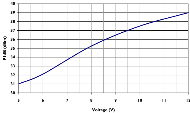
PI dB Vs Voltage 2.5GHz
