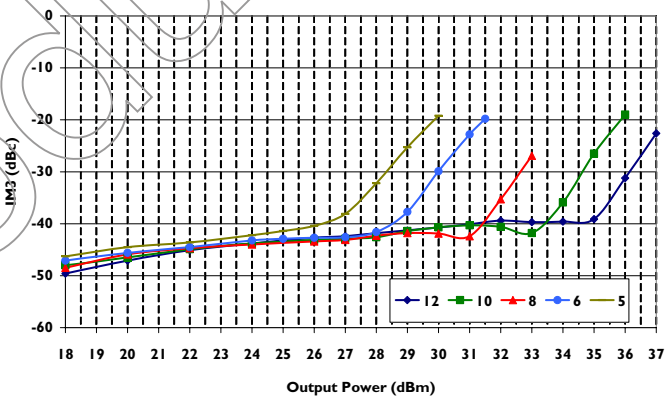
IM3 Vs Output Power Vs Voltage Tone Spacing =100KHz, +12V, 2.5GHz
