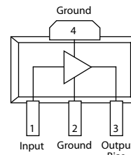
Functional Block Diagram (SOT-89)
