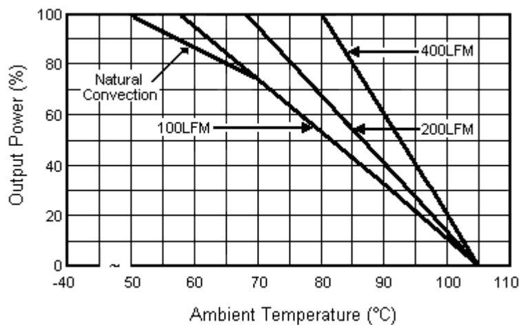
DERATING CURVE
