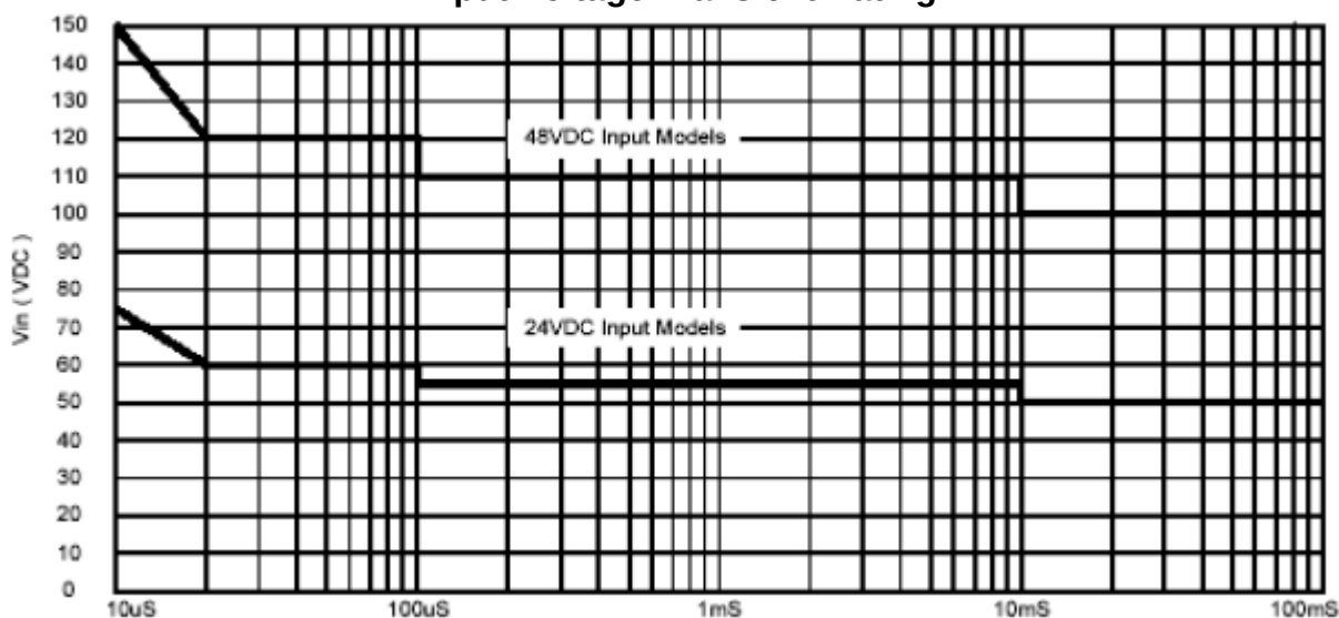
Input Voltage Transient Rating
