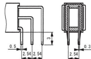
Terminal style of c6 (Style : V/M Terminal)
