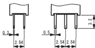
Terminal style of c (Style : PC Terminal)
