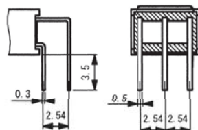
Terminal style of c4 (Style : R/A Terminal)
