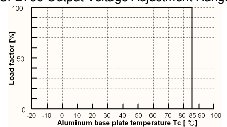
CFB750-300SXX Derating
